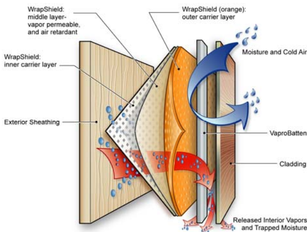
WrapShield membrane construction showing the middle layer as vapor permeable and air retardant. .
